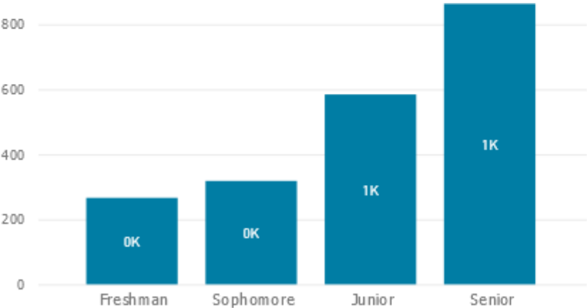
Classification
